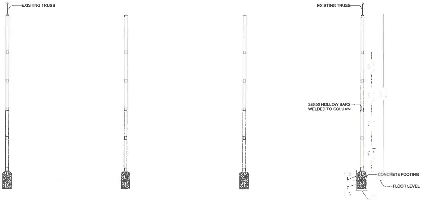
FRONT VIEW
